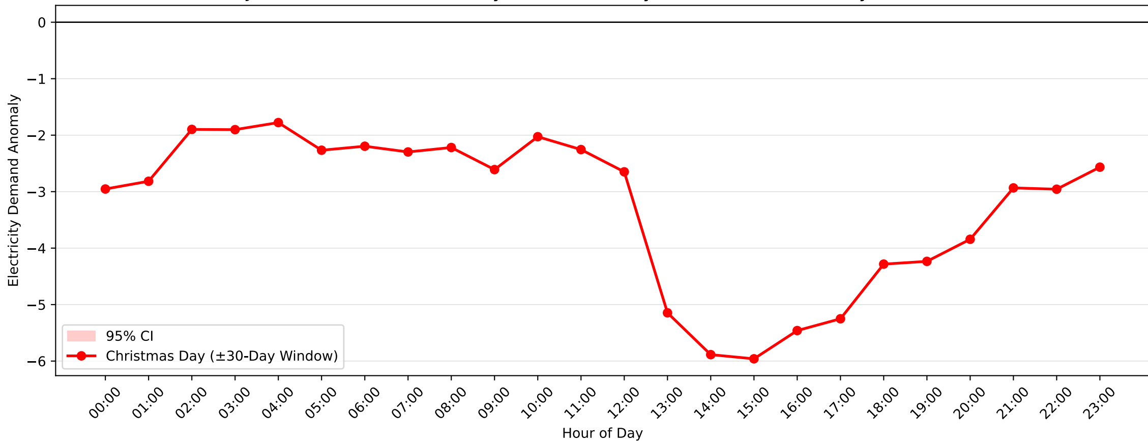
Jesmond Demand Anomaly: Christmas Day (2016–2017, \pm 30 -Day Window)
