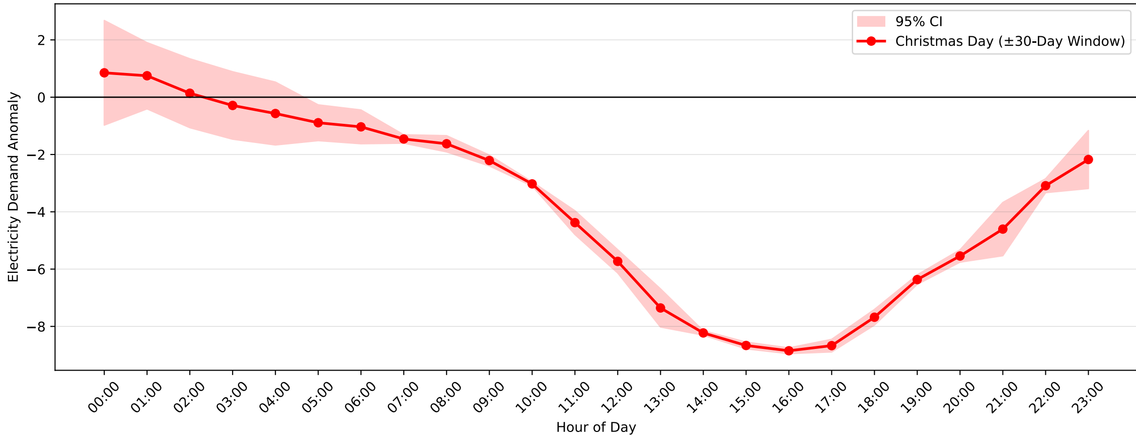
Jesmond Demand Anomaly: Christmas Day (2012-2013, \pm 30 -Day Window)
